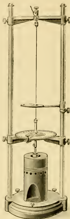
FIG. 98. TORSION VISCOSIMETER Devised by O. S. Doolittle, for use in lab. of Philadelphia and Reading Railroad Co.
