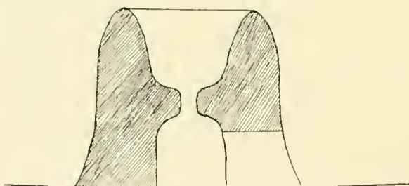
Fig. 48.—Sectional Elevation of Ancient Furnace. Scale: 1/12
