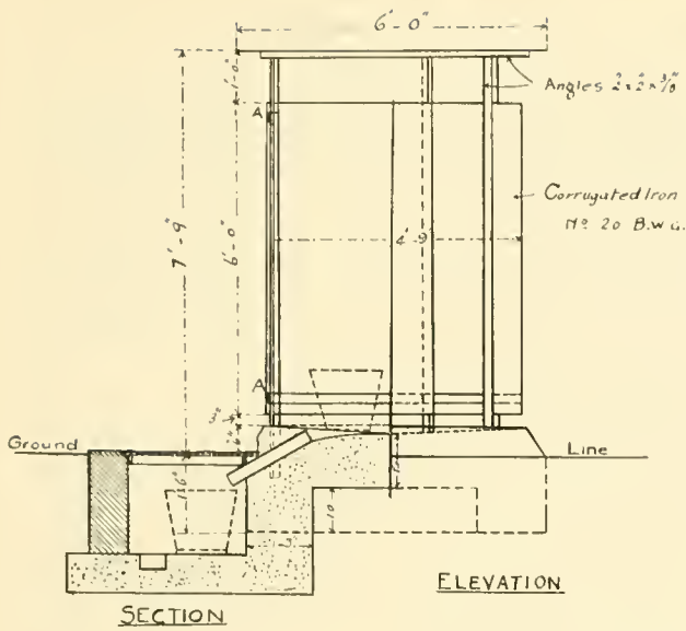
FIG. 98.—PUBLIC URINAL WITH WASH PIT
