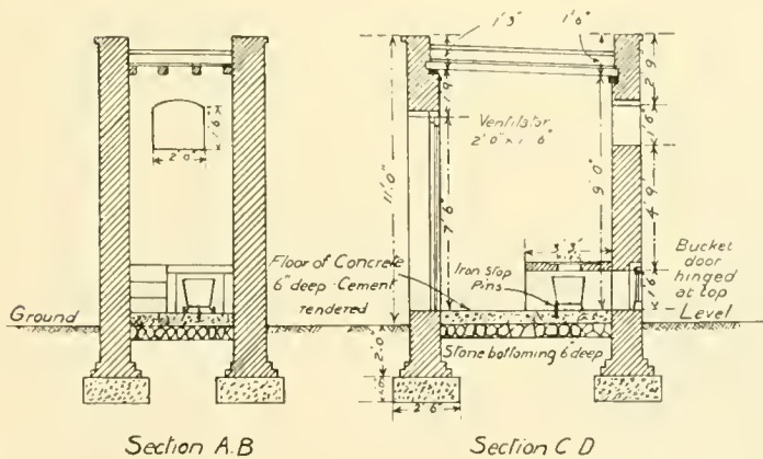
FIG. 99.—TYPE EUROPEAN LATRINE
