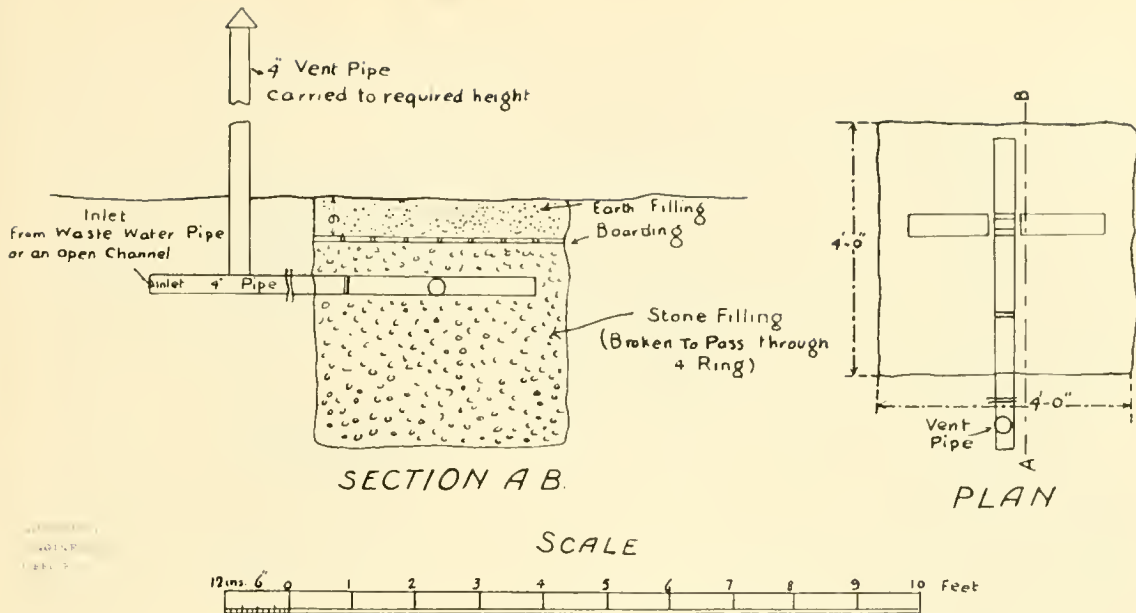
FIG. 92. PERCOLATION PIT
