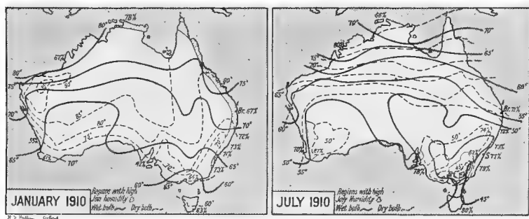
FIG. 19. Typical Climate of Hottest and Coolest Month.
