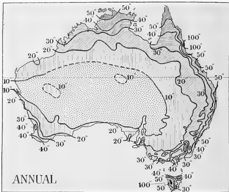
FIG. 24. Mean Annual Rainfall.
