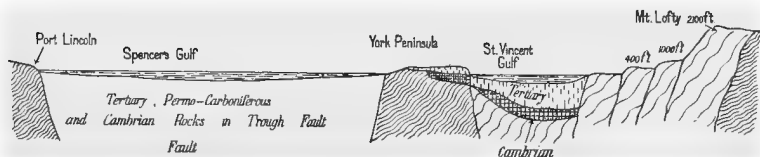
FIG. 13. Section across the Rift Valley of South Australia.
