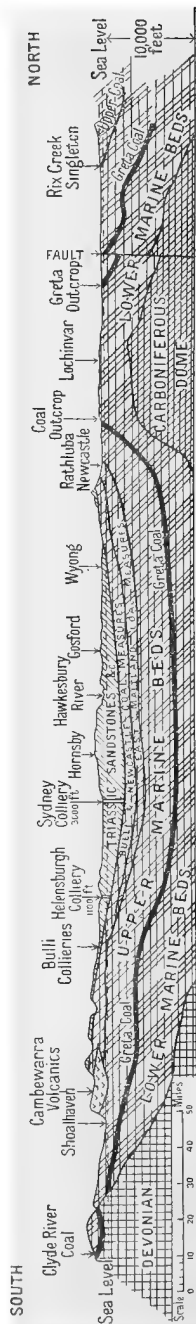
Fig. 53. Section across New South Wales Coal Basin.
