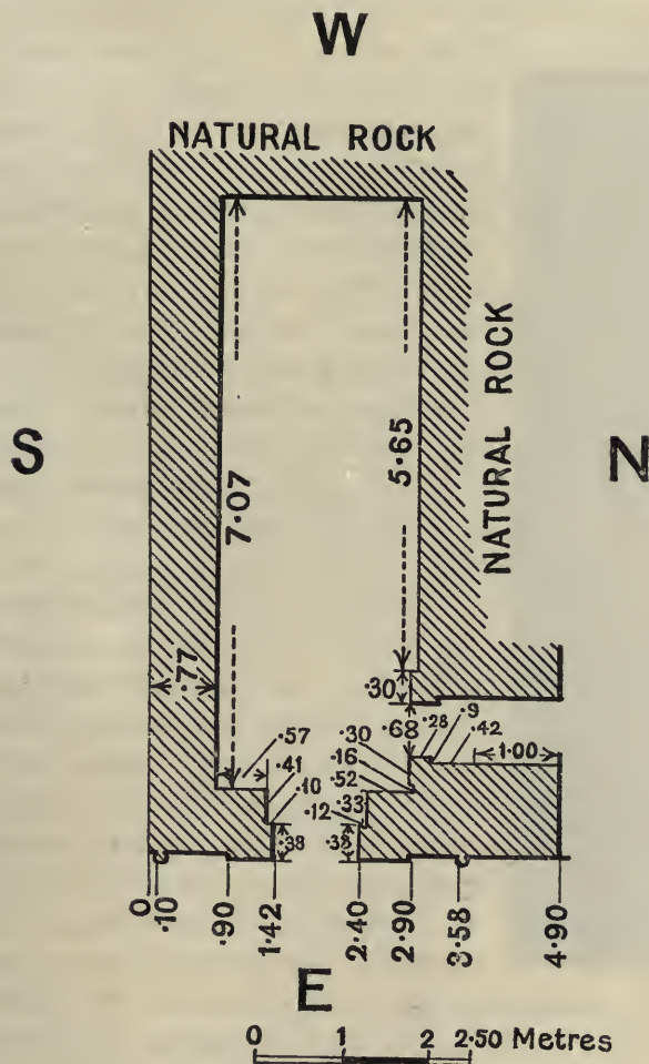
PLAN OF THE TEMPLE OF GAZÎRAT AL-MALIK, DRAWN BY J. W. CROWFOOT, ESQ.
